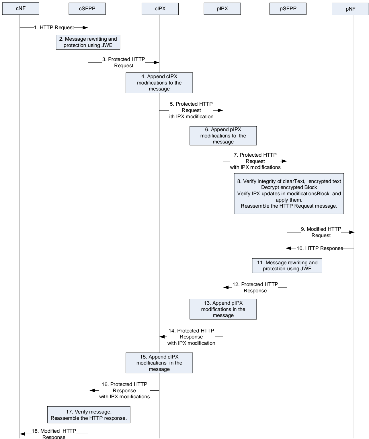
Figure 13.2.4.8-1 Message flow between two SEPPs
